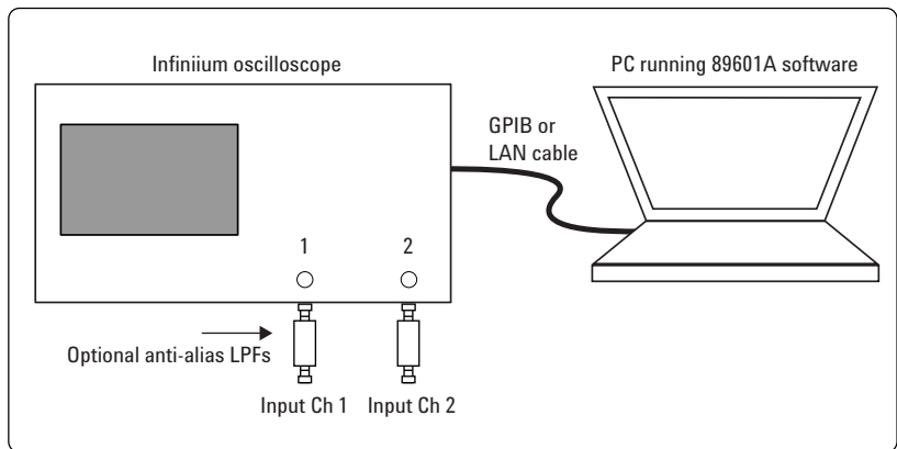
Figure 1a. Equipment connections for 2-channel oscilloscopes
