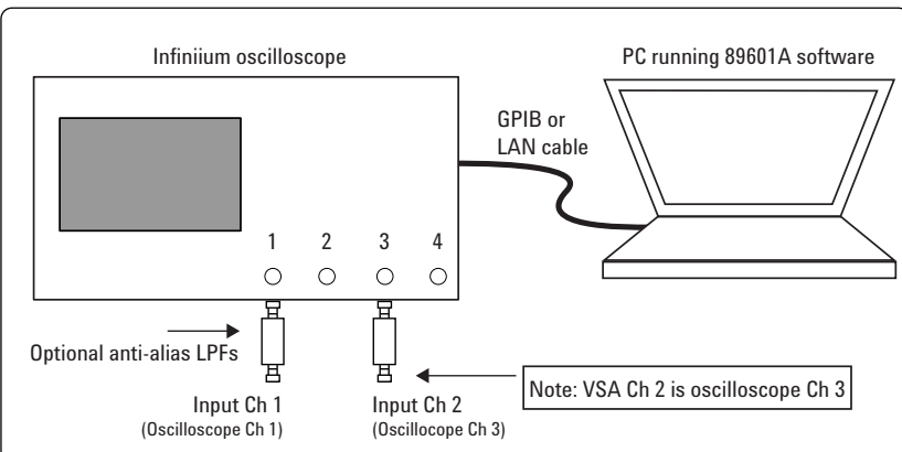
Figure 1b. Equipment connections for 4-channel oscilloscopes
